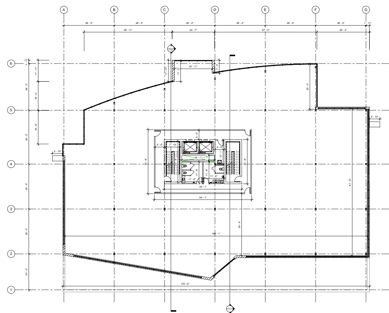
1 2ND FLOOR 1/8" = 1'-0"
